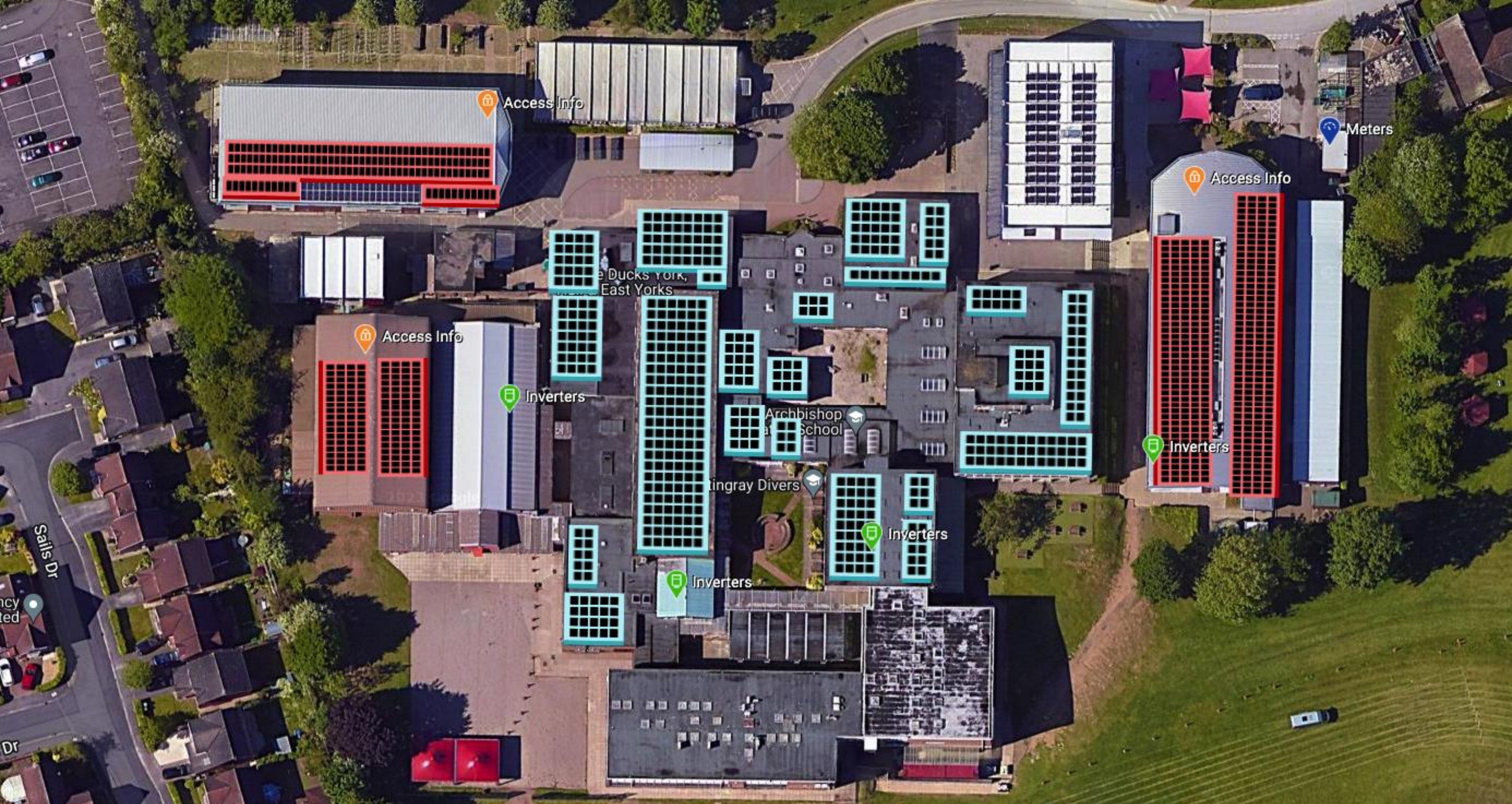
Archbishop Holgate, built in September, is the largest system we have completed to date at: 460.1kW (plus existing system)
